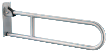
A1599D bathroom flip up grab bar heavy duty stainless steel 304 size: 805x100x260mm tube: dia. 32x1.2mm thickness
